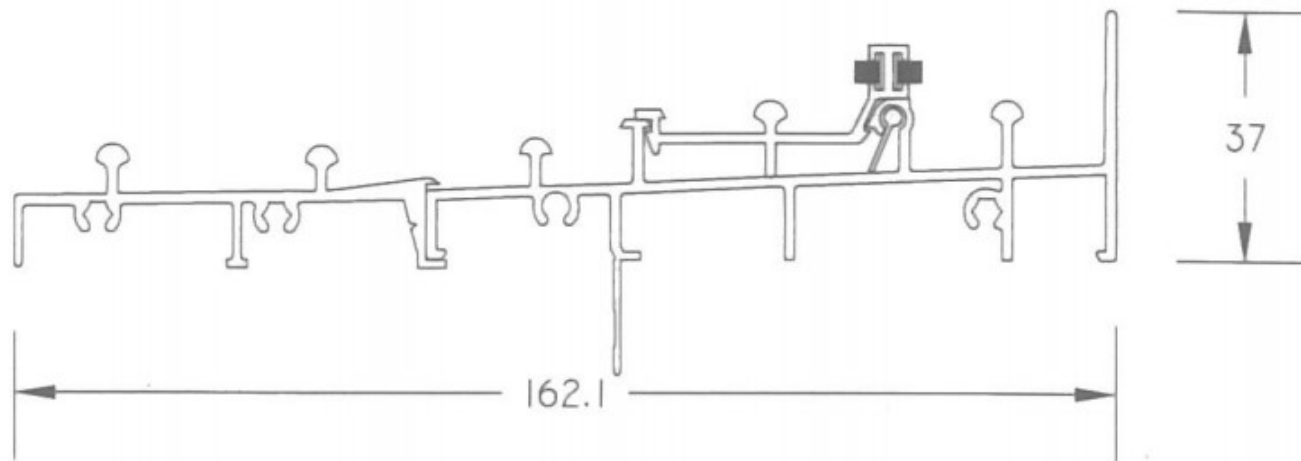
QUANTUM STACKER SLIDING DOOR SILL WITH FLYDOOR TRACK
