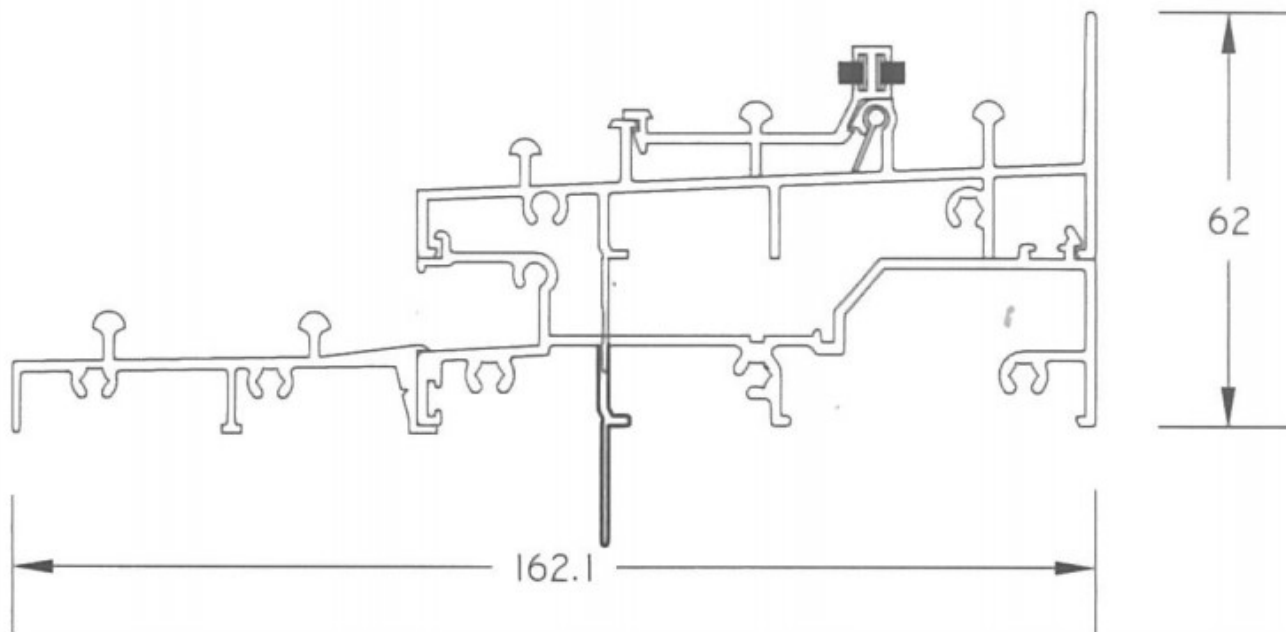
QUANTUM STACKER SLIDING DOOR SILL WITH FLYDOOR TRACK WITH SUMPSILL
