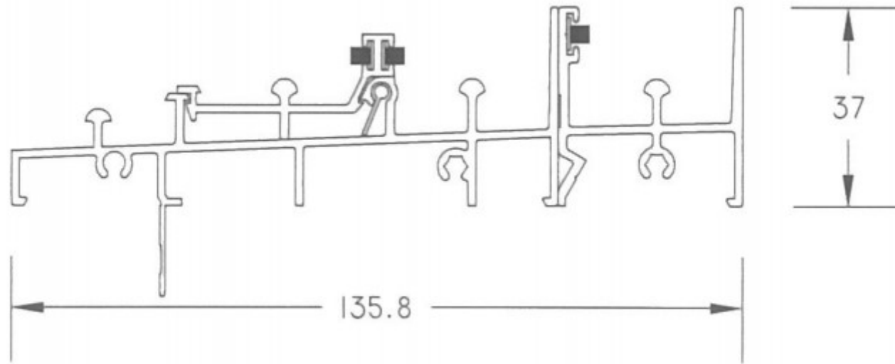
QUANTUM FOUR PANEL STACKER SLIDING DOOR SILL
