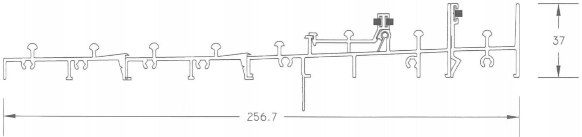
QUANTUM FOUR PANEL STACKER SLIDING DOOR SILL WITH FLYDOOR TRACKS
